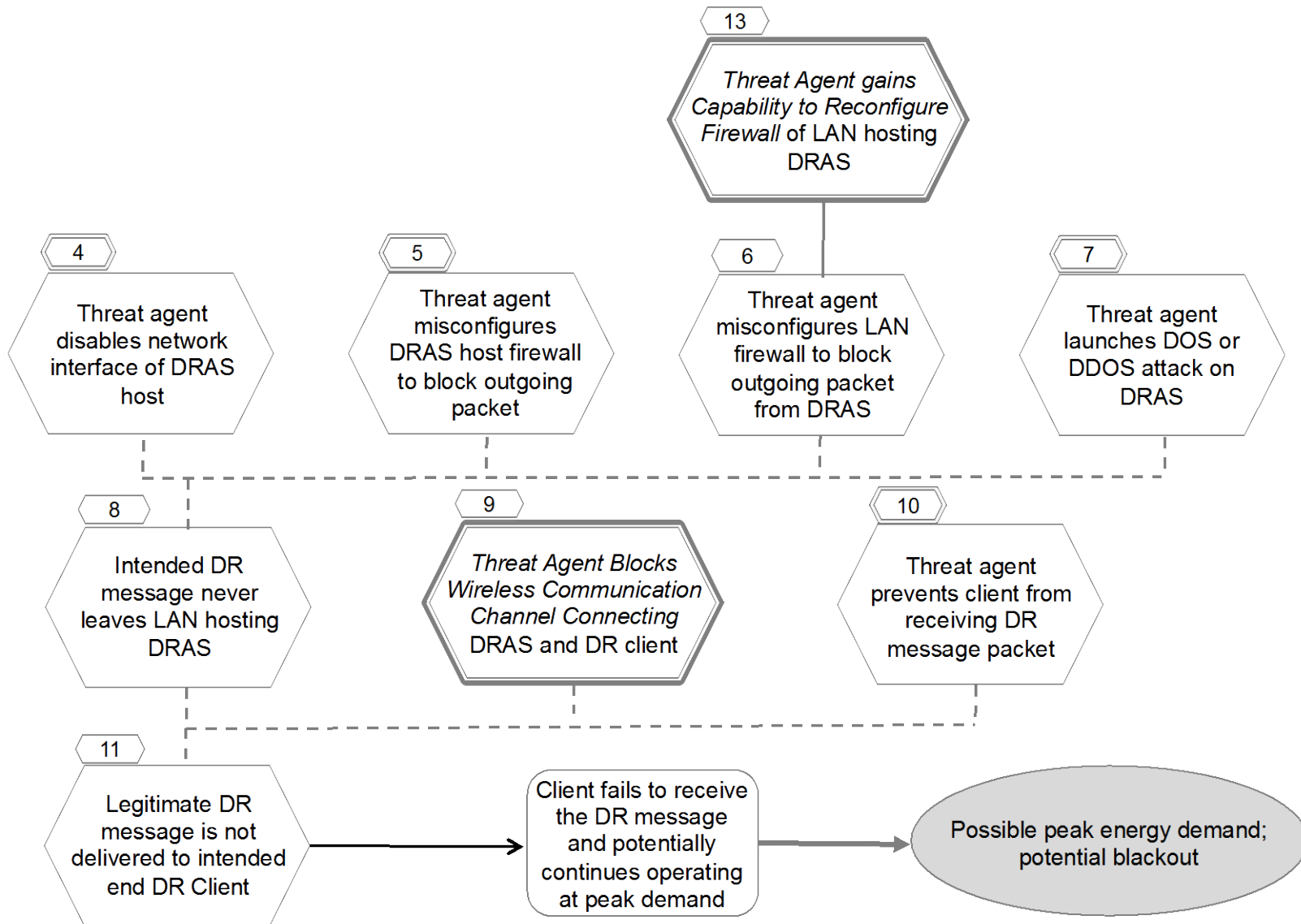
Figure 19 - Blocked DR Messages Result in Increased Prices or Outages (3/8)
