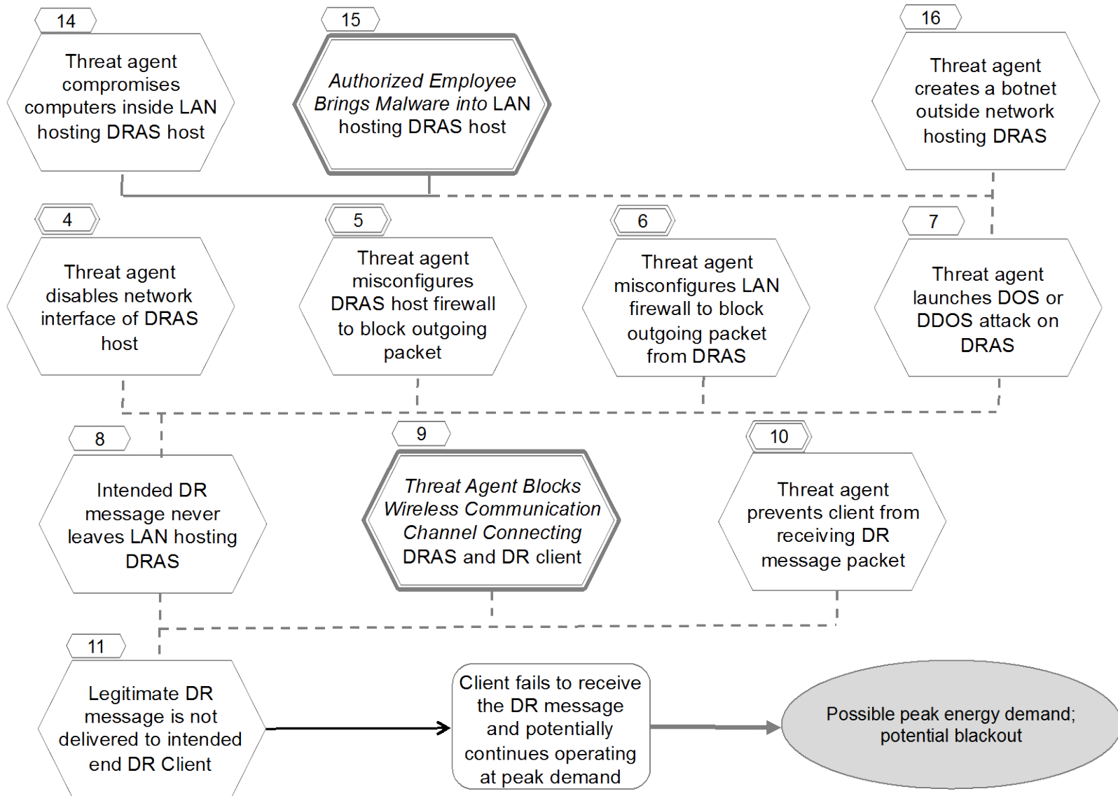
Figure 20 - Blocked DR Messages Result in Increased Prices or Outages (4/8)
