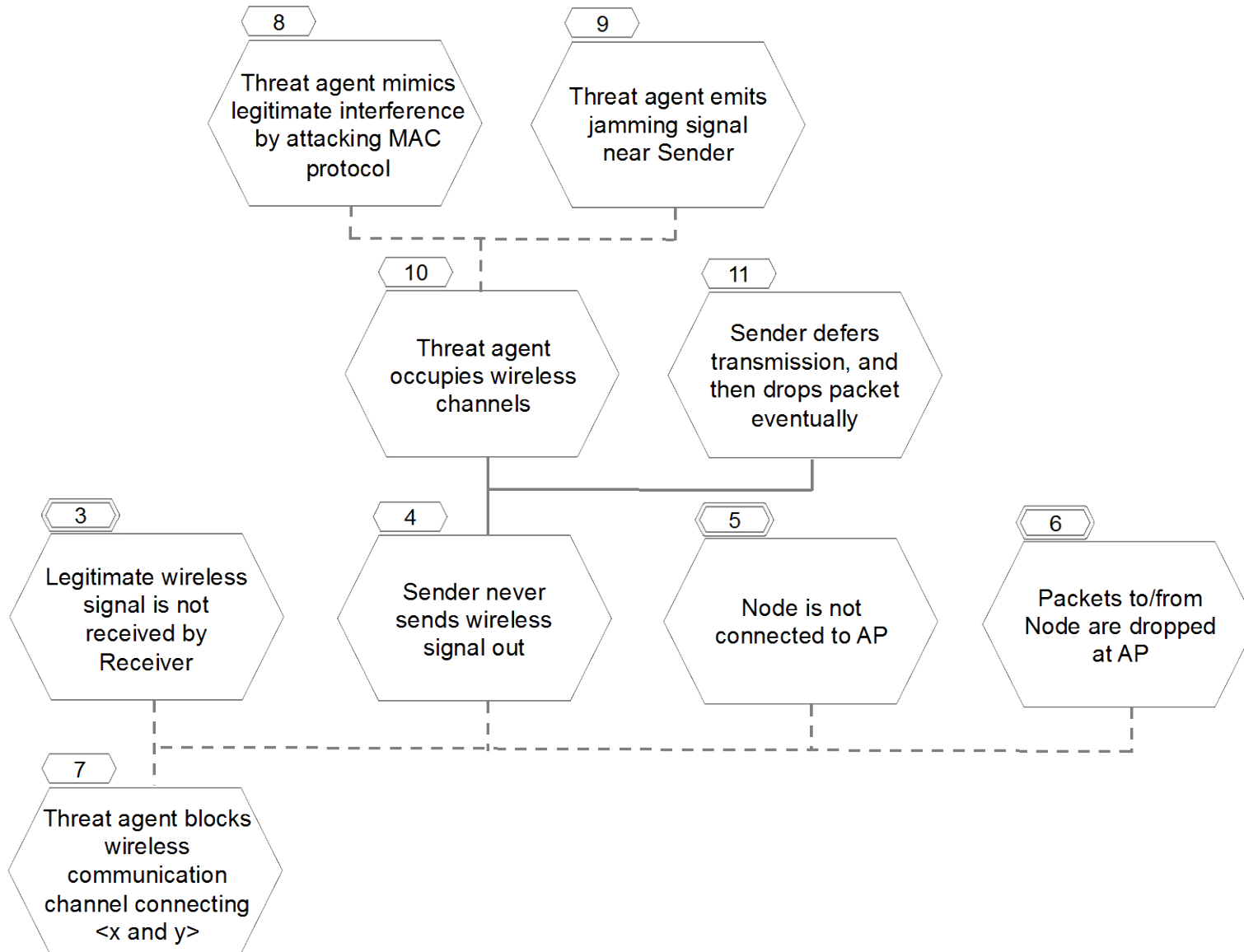
Figure 32 - Threat Agent Blocks Wireless Communication Channel (2/4)
