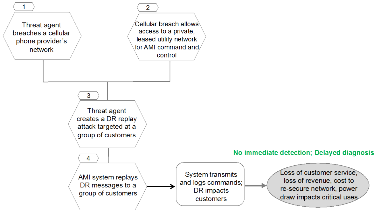
Figure 12 - Breach of Cellular Provider's Network Exposes AMI Access
