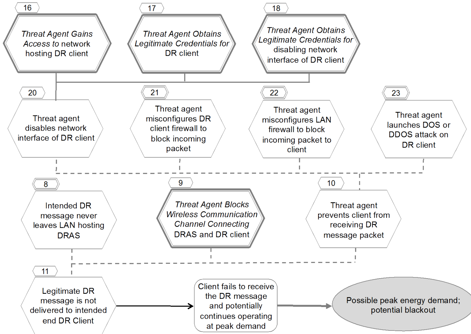
Figure 21 - Blocked DR Messages Result in Increased Prices or Outages (5/8)
