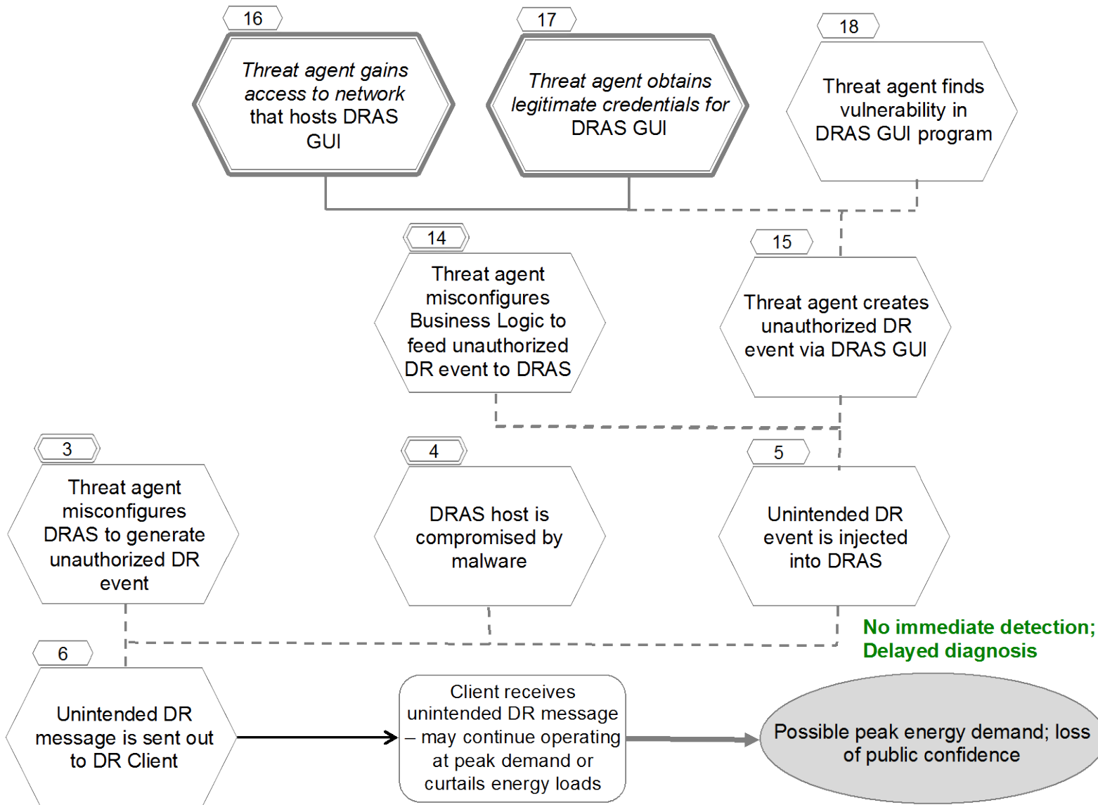
Figure 29 - Improper DRAS Configuration Causes Inappropriate DR Messages (4/4)
