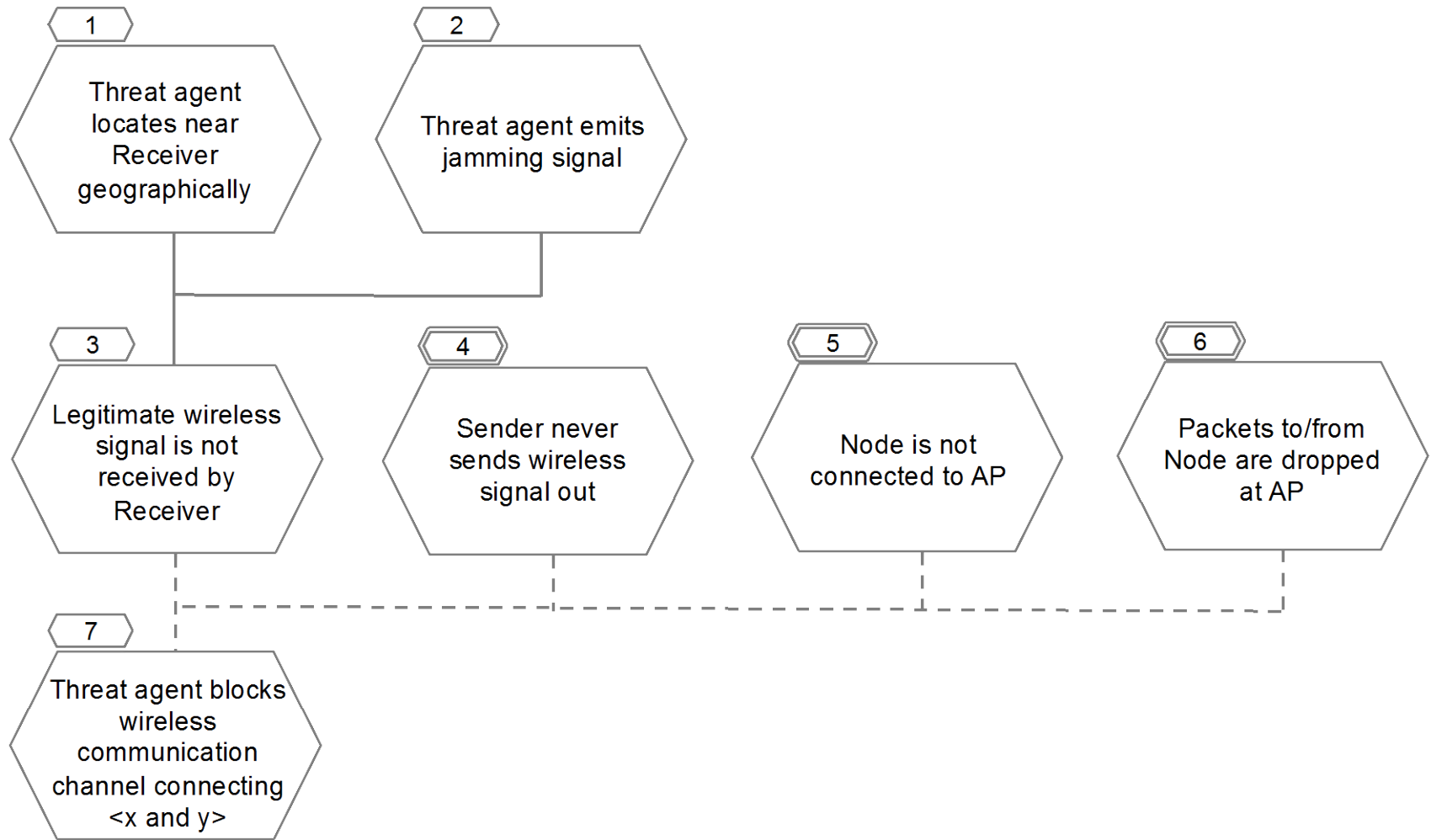
Figure 31 - Threat Agent Blocks Wireless Communication Channel (1/4)
