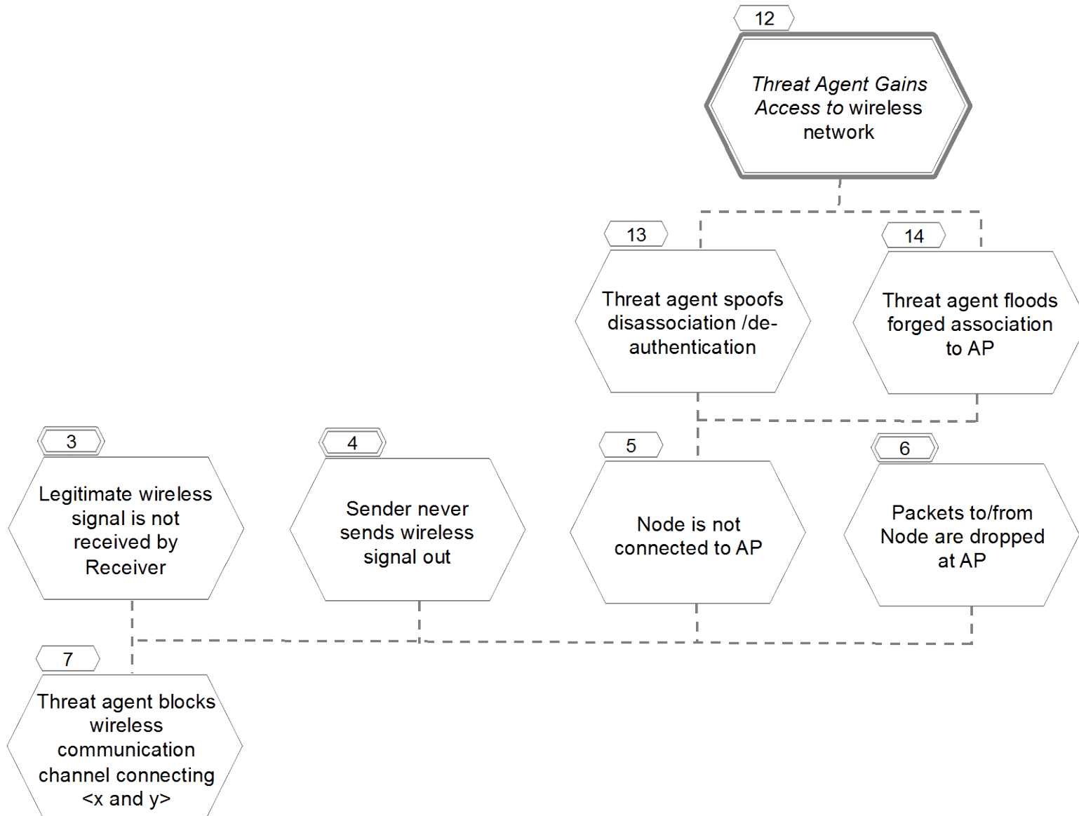
Figure 33 - Threat Agent Blocks Wireless Communication Channel (3/4)
