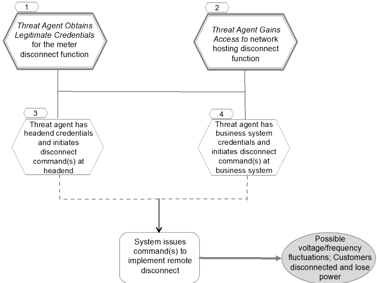
Figure 10 - Invalid Disconnect Messages to Meters Impact Customers and Utility
