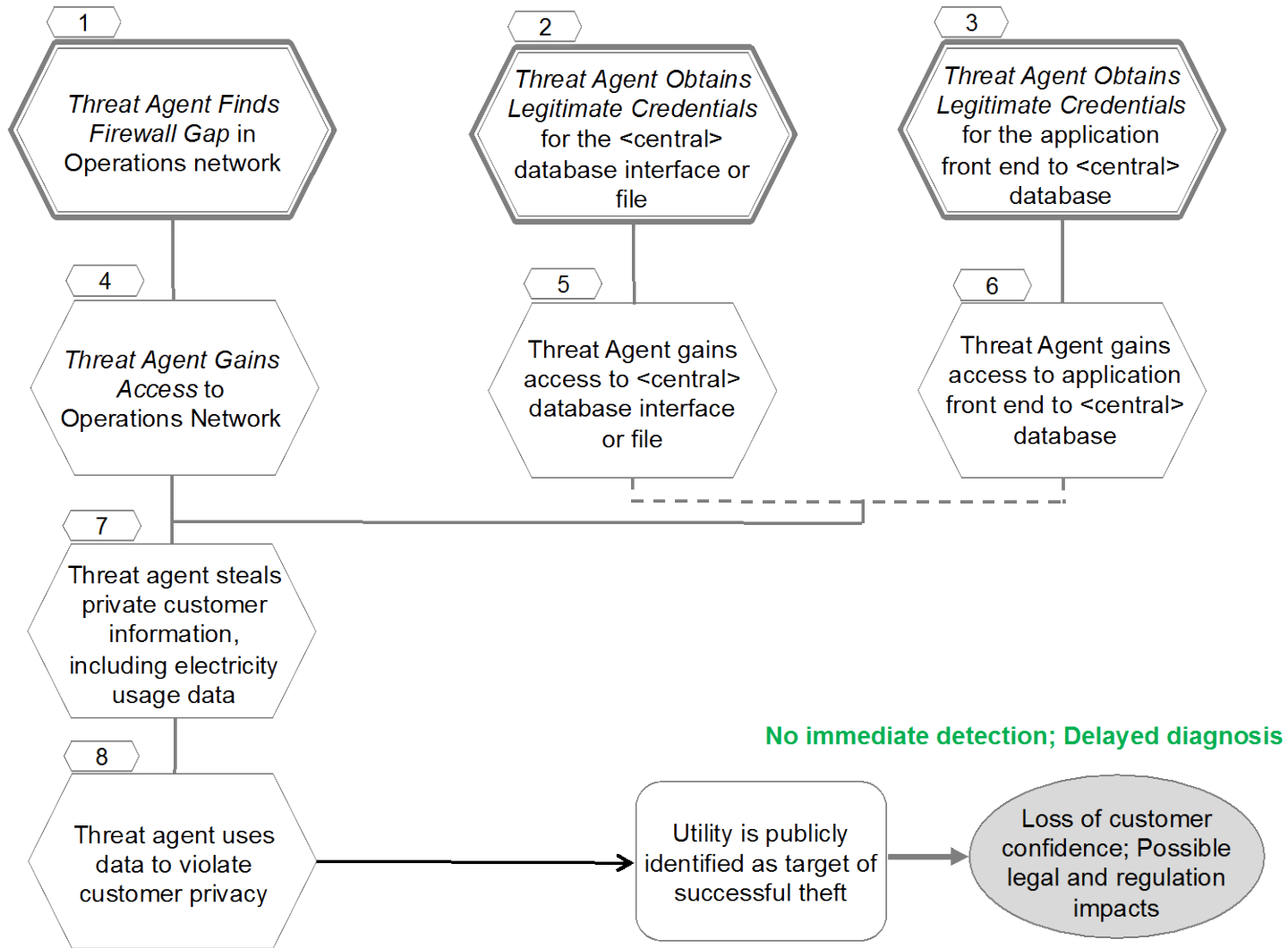
Figure 11 - Improper Firewall Configuration Exposes Customer Data
