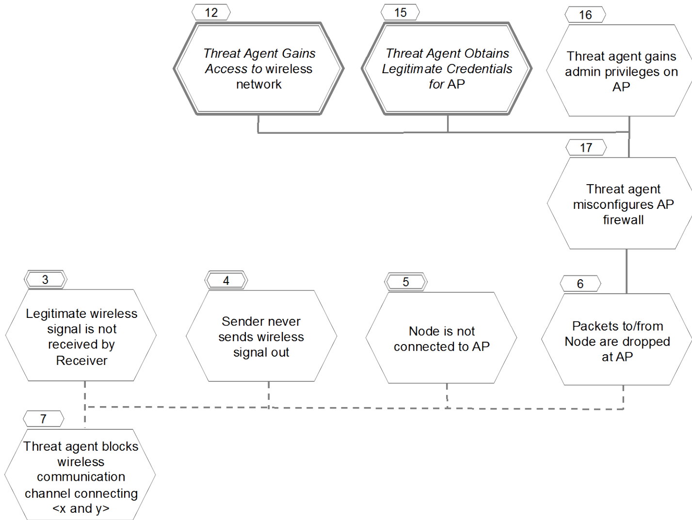
Figure 34 - Threat Agent Blocks Wireless Communication Channel (4/4)
