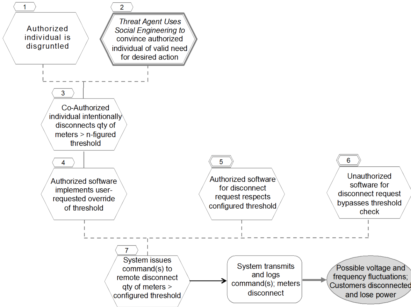
Figure 2 - Mass Meter Remote Disconnect by Authorized Individual (1/3)
