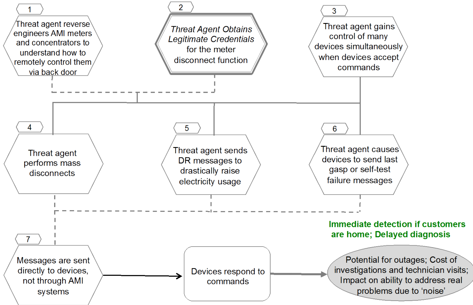
Figure 14 - Reverse Engineering of AMI Equipment Allows Unauthorized Mass Control
