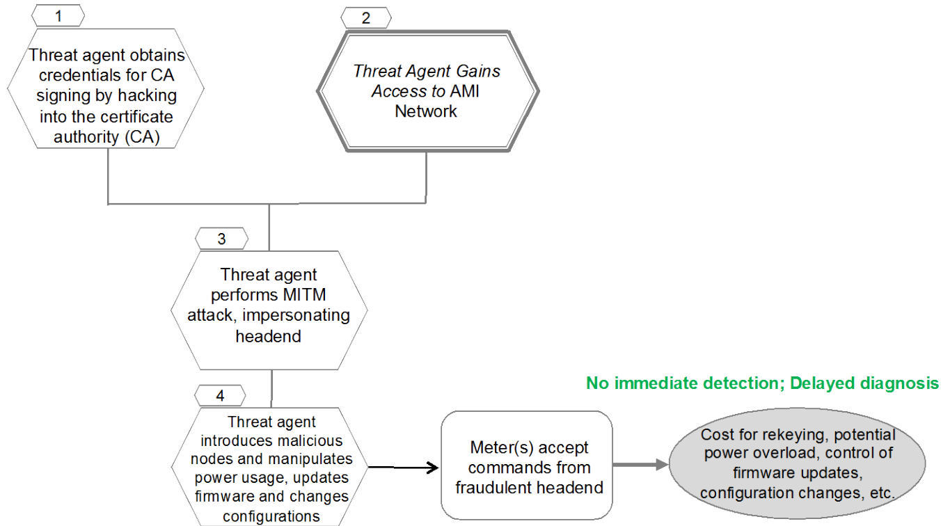
Figure 13 - Compromised Headend Allows Impersonation of CA
