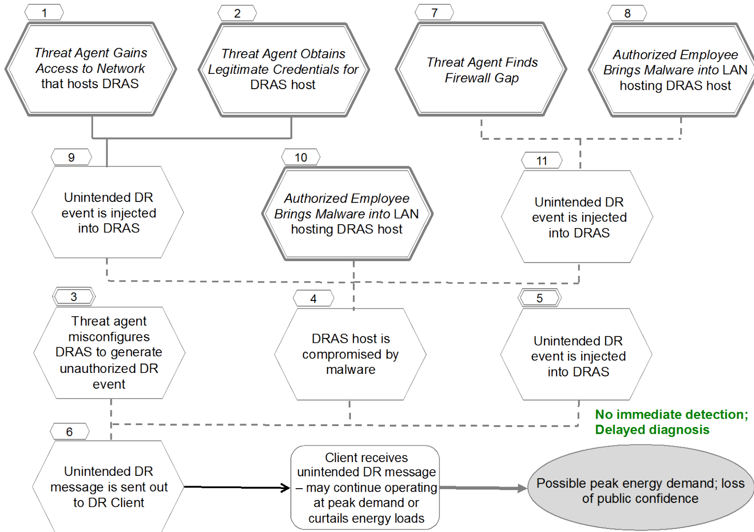
Figure 27 - Improper DRAS Configuration Causes Inappropriate DR Messages (2/4)
