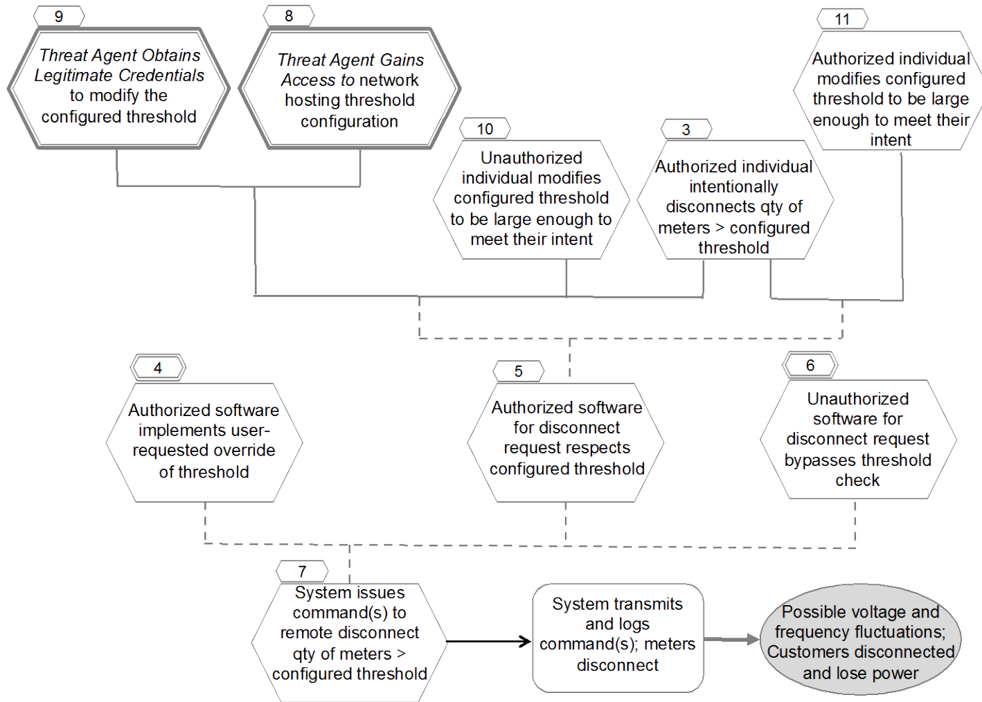
Figure 3 - Mass Meter Remote Disconnect by Authorized Individual (2/3)
