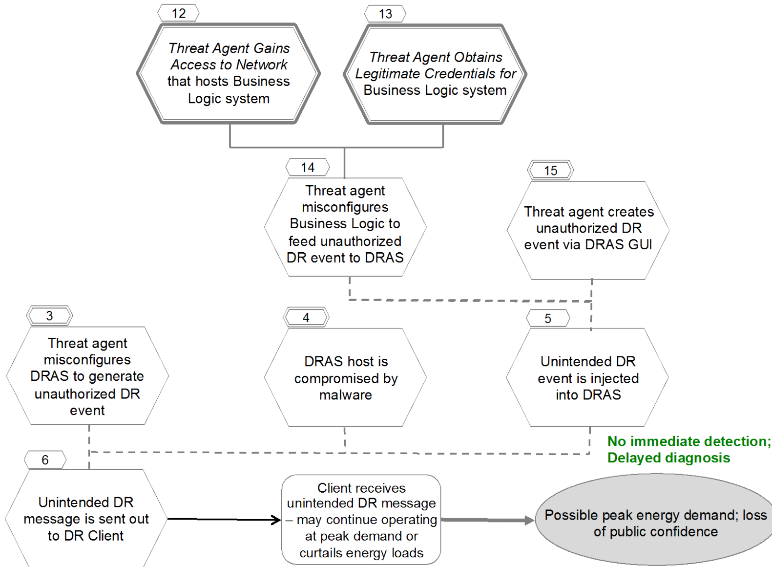
Figure 28 - Improper DRAS Configuration Causes Inappropriate DR Messages (3/4)
