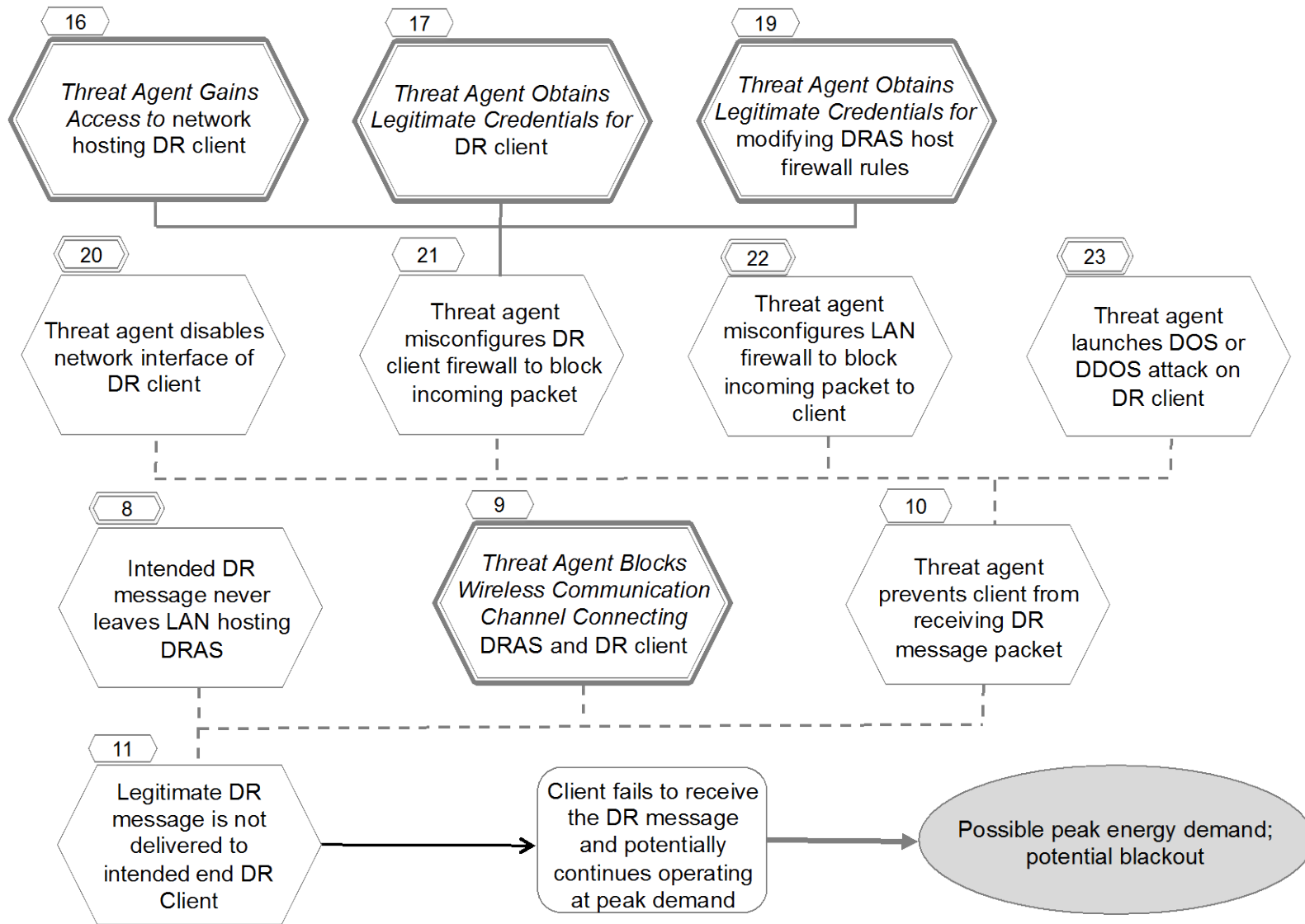
Figure 22 - Blocked DR Messages Result in Increased Prices or Outages (6/8)
