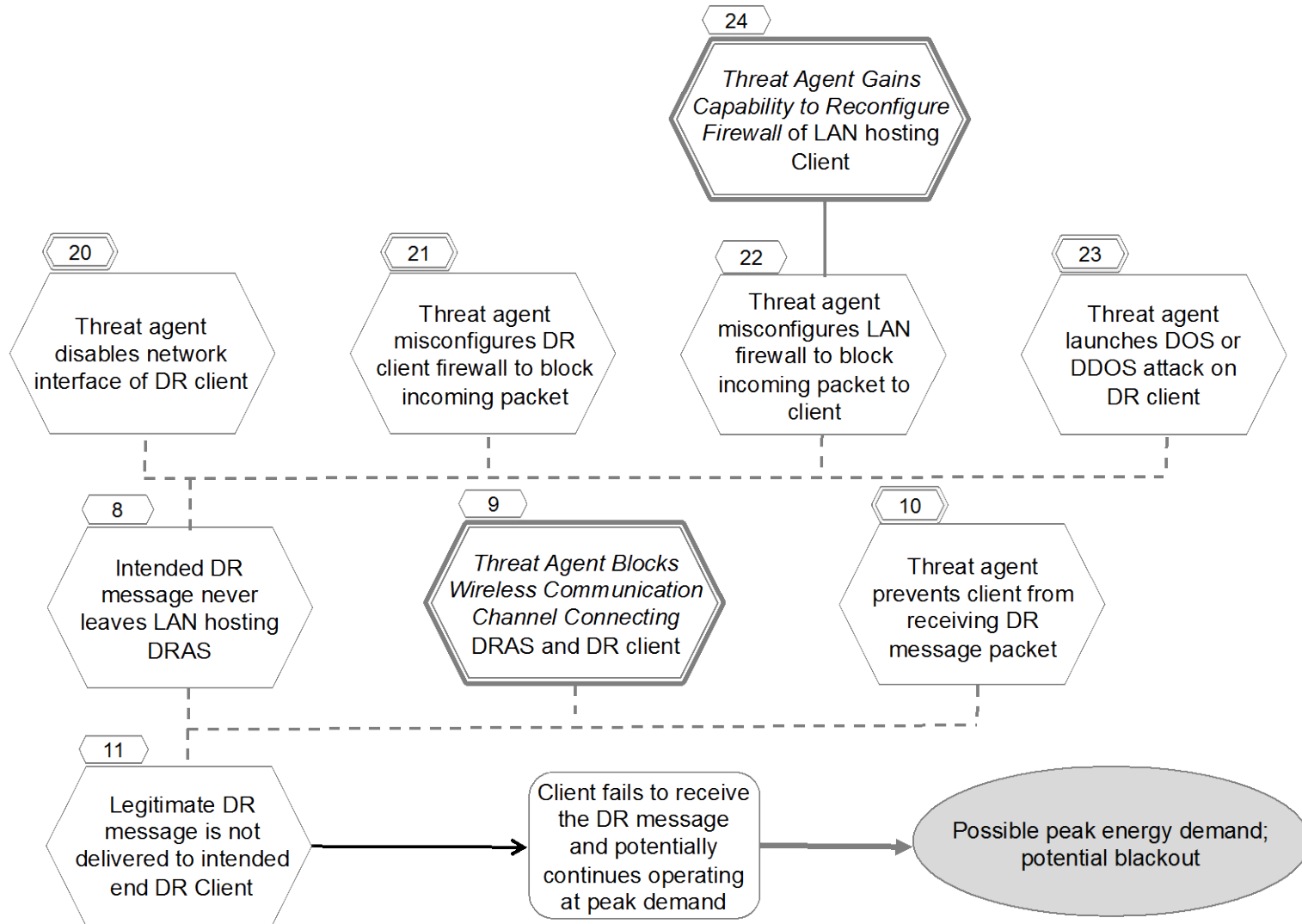
Figure 23 - Blocked DR Messages Result in Increased Prices or Outages (7/8)
